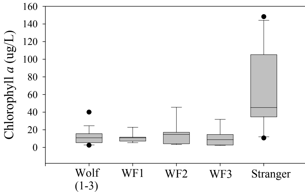
Figure 19. Box plots comparing chlorophyll a (ug/L) concentrations from the three Wolf Creek sites and Stanger Creek.
