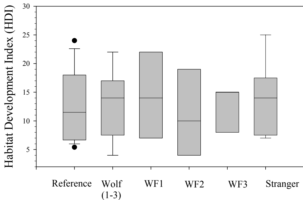
Figure 22. Box plots comparing Habitat Development Index (HDI) at Wolf Creek (all three sites combined) and reference streams. Data was also plotted from each Wolf Creek site separately in order to make comparisons between the three sites, and from Stranger Creek.
