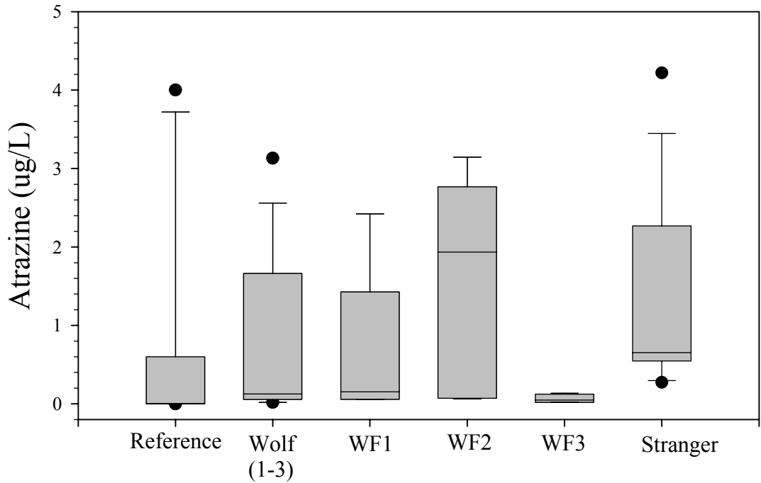
Figure 17. Box plots comparing atrazine (ug/L) at WolfCreek (all three sites combined) and reference streams. Data was also plotted from each Wolf Creek site separately in order to make comparisons between the three sites, and from Stanger Creek.
