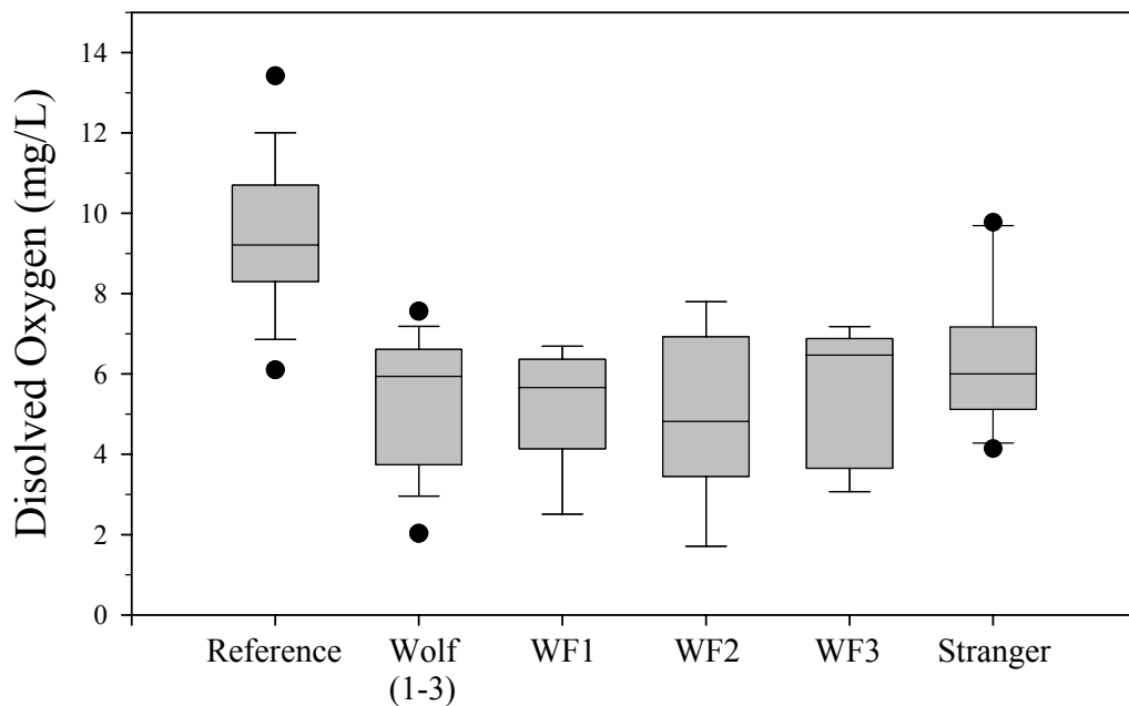
Figure 10. Box plots comparing dissolved oxygen (mg/L) at Wolf Creek (all three sites combined) and reference streams. Data was also plotted from each Wolf Creek site separately in order to make comparisons between the three sites, and from Stanger Creek.
