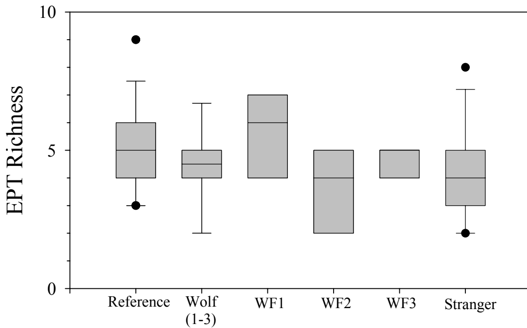
Figure 24. Box plots comparing EPT richness at Wolf Creek (all three sites combined) and reference streams. Data was also plotted from each Wolf Creek site separately in order to make comparisons between the three sites, and from Stranger Creek.
